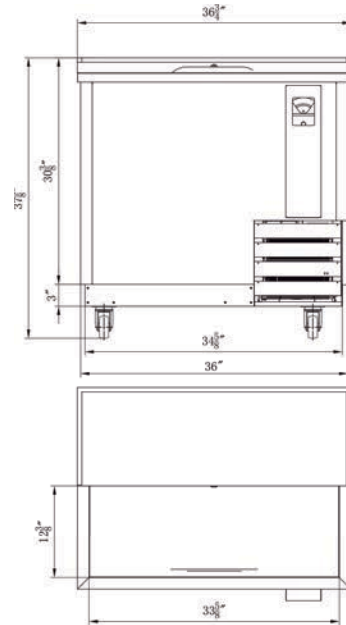
DHBC36 Front View
