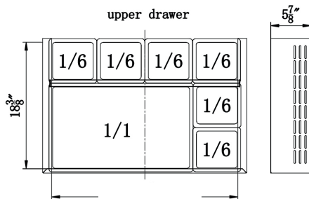
Upper drawer
