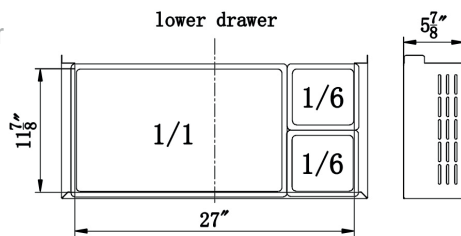
Lower drawer
